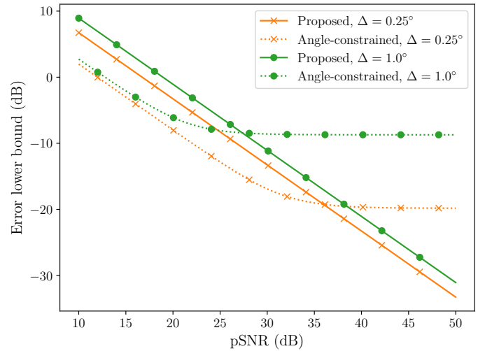
Fig. 2. Comparison of estimation strategies for multipath channels generated according to NYUSIM channel model [40]. Averages over 1000 channel realizations are shown.
