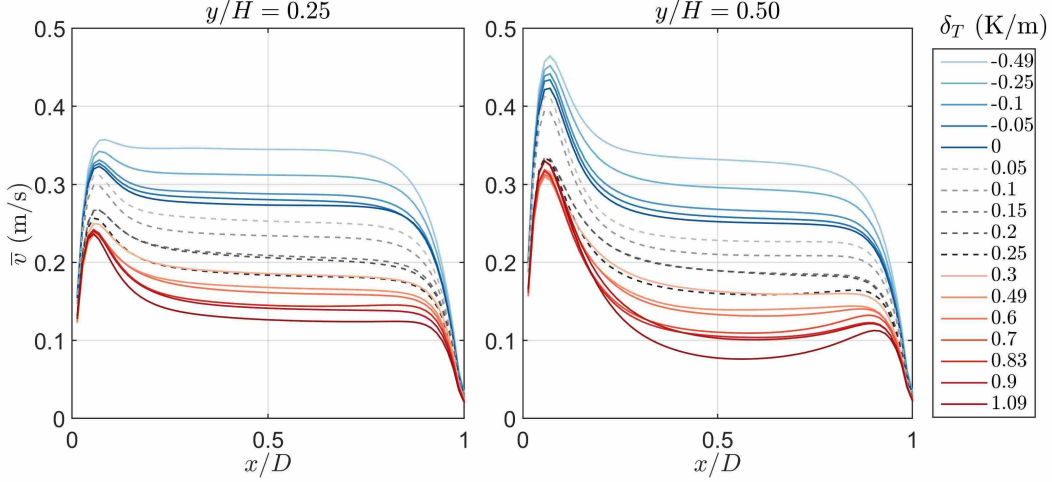
Figure .13: Time-averaged velocity in the mid-plane at z/W=0.5 and at heights y/H=0.25 , y/H=0.5 for various external thermal stratification at Ra = 1.5 \times 10^{12} .
