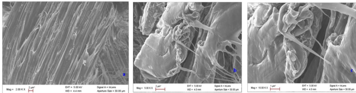
Figure 5. SEM pictures of PE-C. Fornicata coated with SA.
