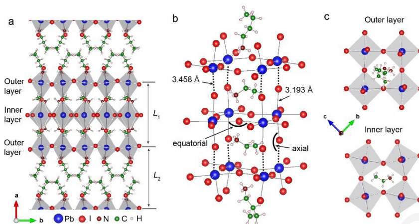
Figure 1. The crystal structure of (\text{BA})_2(\text{EA})_2\text{Pb}_3\text{I}_{10} . (a) Side-view of the crystal structure along c direction. Also illustrated are the definition of the thickness of perovskite slab ( L_1 ) and the interlayer distance ( L_2 ). (b) Crystal structure of the perovskite cages showing the occupation of the EA cations in the cuboctahedral sites. The dash lines highlight the longest Pb-I bonds. Also illustrated are the definition of equatorial and axial Pb-I-Pb angles. (c) Top-view of the outer layer and inner layer, which clearly shows different in-plane tilt.
