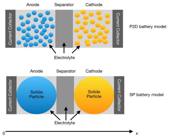
Figure 1: P2D and single particle battery model
