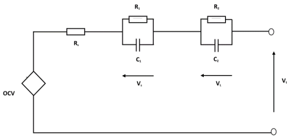
Figure 2 : Second order equivalent circuit model
