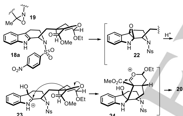
Scheme 4. Bottom and side views of DFT-minimized conformation of 18a in \text{CH}_2\text{Cl}_2 (Gaussian 09 software package, M06 functional and 6-31G(d,p) basis set for all atoms) and mechanistic hypothesis for the conversion of 18a into 20 .
