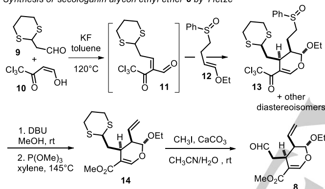
Synthesis of secologanin aglycon ethyl ether 8 by Tietze
