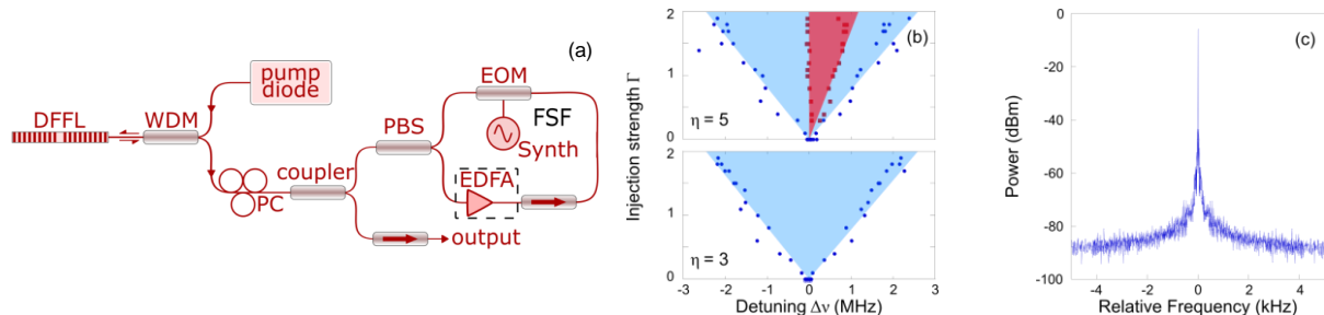
Fig. 1 (a) Experimental scheme. The optional EDFA permits here to control the re-injected power. (b) Normalized injection strength \Gamma with respect to the detuning \Delta\nu at two different excitation ratio \eta . Colored areas delimit the different regimes. White: unlocked, blue: locked, red: chaotic. (c) RF Spectrum of the locked DFFL beat frequency.
