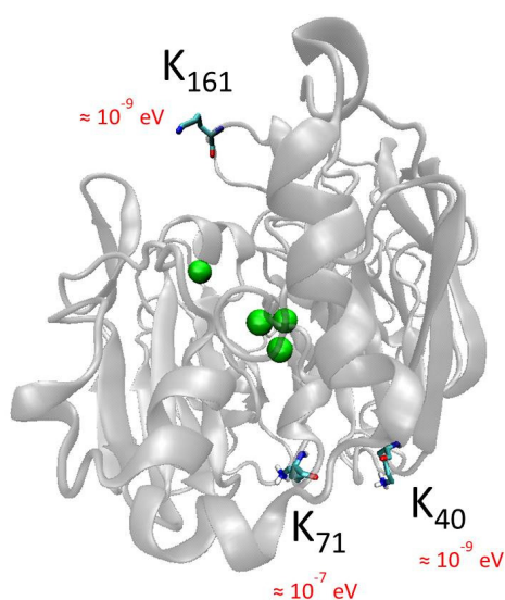
Figure 1. Model of the structure of LAC3 with the three possible locations of lysine in either the native enzyme (K 71 and K 40 ) or its variants UNIK 161 and UNIK 71 . View generated with PyMol. In silico evaluated electronic coupling values from an electron donating surface to the TNC (in eV) are added in red (see text for details).
