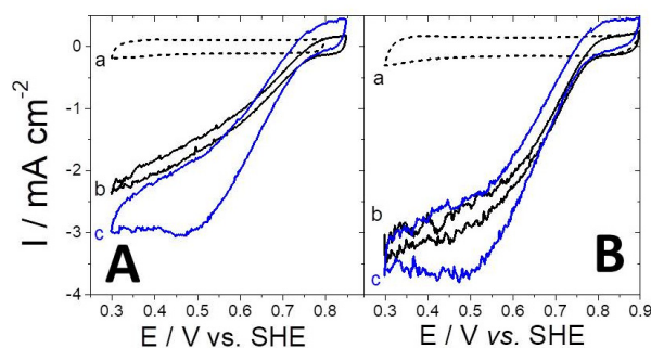
Figure 4. CV of alkyne-UNIK 161 MWCNT electrodes after the spontaneous (A) or the electro grafting (5 CV scans) of 4-azidobenzene diazonium tetrafluoroborate (B). CVs obtained (a) under Ar, (b) under O 2 and (c) after the addition of 10 mM ABTS (0.05 mol L -1 acetate buffer solution pH 5, v = 10 mV s -1 ).
