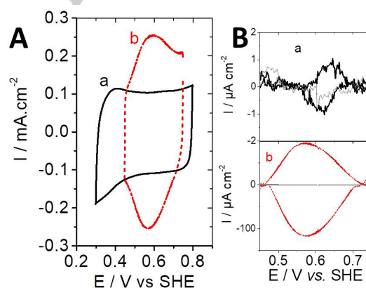
Figure 3. (A) CVs and (B) background-subtracted CVs of (a) alkyne-UNIK 161 and (b)- ethynylferrocene functionalized MWCNT electrodes under argon at pH = 5. The gray line corresponds to a non-modified MWCNT electrode ( 0.05 \text{ mol L}^{-1} in acetate buffer solution, v = 10 \text{ mV s}^{-1} ).
