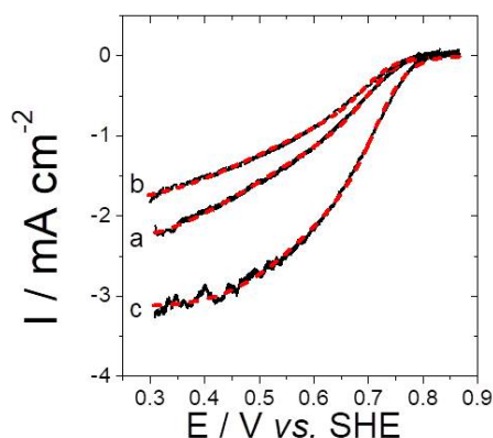
Figure 6. Background-subtracted CV of (alkyne) 2 -LAC3 (a), alkyne-UNIK 161 (b) and alkyne-UNIK 71 (c) functionalized MWCNT electrodes under O 2 and respective simulated CV scan (red trace) (0.05 mol L -1 acetate buffer solution pH 5, \nu = 10 mV s -1 ). Background-subtracted CVs take into account the average between the backward and forward CV scans.
