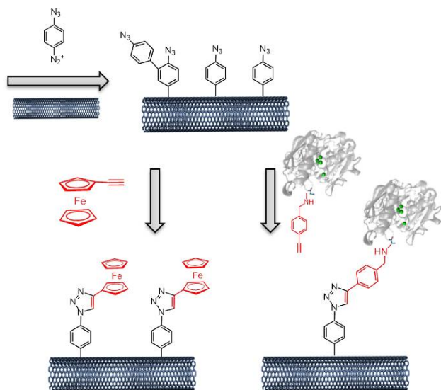
Figure 2. Schematic representation of the covalent modification of CNT by click chemistry of ferrocene-alkyne and alkyne modified LAC3 variants.
