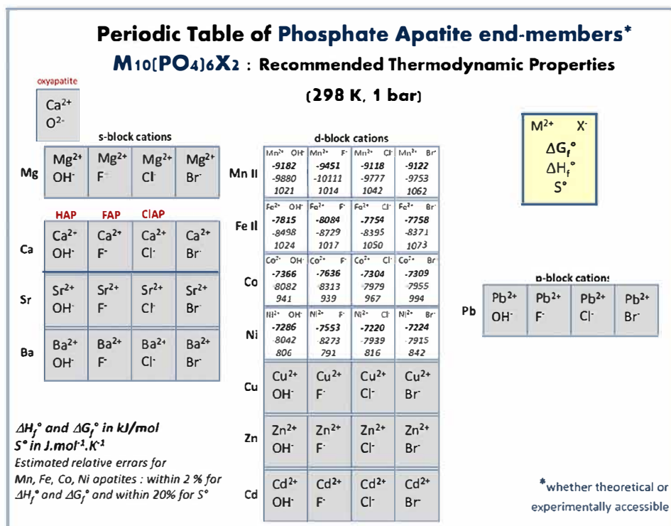
FIGURE 2. Periodic table summarizing recommended thermodynamic values (at T = 298\text{ K} , 1 bar), for theoretical \text{M}_{10}(\text{PO}_4)_6\text{X}_2 end-members with \text{M} = \text{Ni} , \text{Co} , \text{Mn}(\text{II}) or \text{Fe}(\text{II}) and \text{X} = \text{OH} , \text{F} , \text{Cl} or \text{Br} . The shaded zones have already been reported previously (see Table 5 in reference [11]) and therefore were not detailed here.
