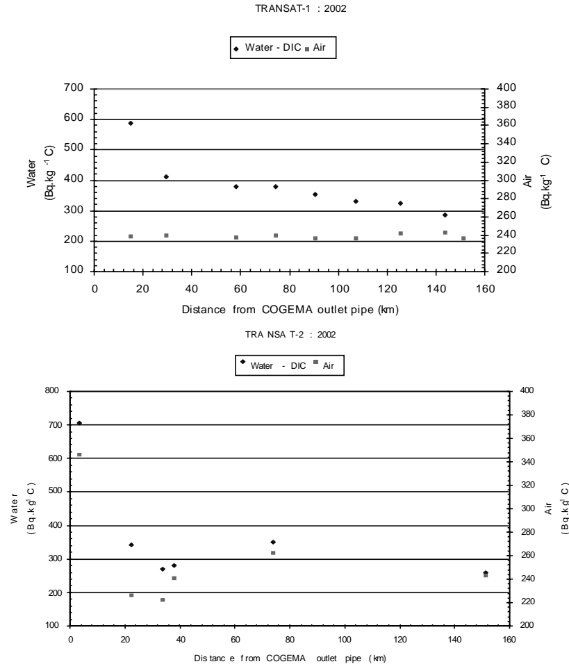
Figure 5 Variations of ^{14}\text{C} activities ( \text{Bq}\cdot\text{kg}^{-1}\text{C} ) in surface seawater and air versus distance from pipe outlet during TRANSAT 1(above) and 2 (below) cruises
