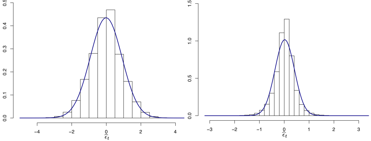
FIGURE 1. Histograms for the estimated errors \widehat{\epsilon}_t of Experiment 1 (left) and Experiment 2 (right).
