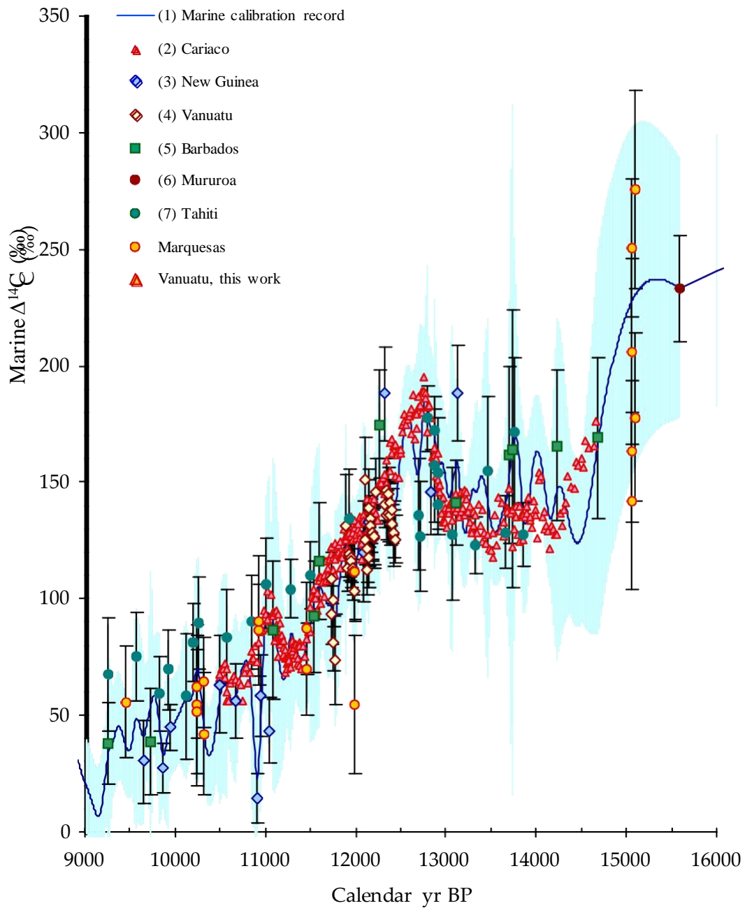
Figure 5 Marine \Delta^{14}\text{C} changes at the 2\text{-}\sigma confidence level as a function of calendar ages. The blue envelope figured out the 2\text{-}\sigma error of the marine INTCAL98 \Delta^{14}\text{C} values. (1) Stuiver et al 1998; (2) Hughen et al. 2000; (3) Edwards et al. 1993; (4) Burr et al. 1998; (5, 6, 7) Bard et al. 1993, 1998. Same references as Figure 2.
