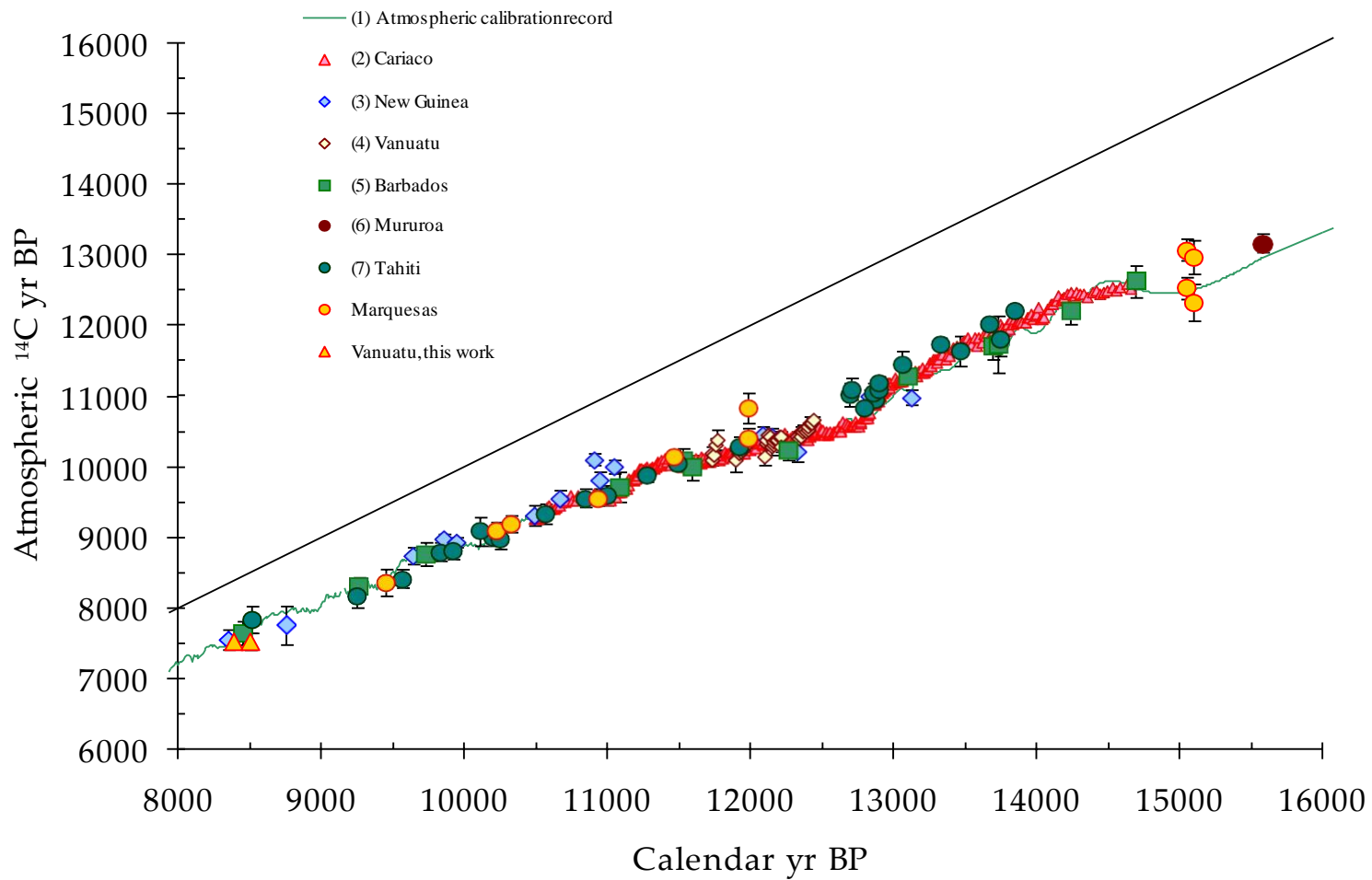
Figure 2 Atmospheric ^{14}\text{C} ages (error bars at 2\sigma ) as a function of calendar ages (error bars not represented). Calendar ages refer to ^{230}\text{Th}/\text{U} dating. (1) Stuiver et al 1998; (2) Hughen et al. 2000; (3) Edwards et al. 1993; (4) Burr et al. 1998; (5, 6, 7) Bard et al. 1993, 1998. The ^{14}\text{C} ages of the Marquesas and Vanuatu corals were corrected for a reservoir age of 400 yr.
