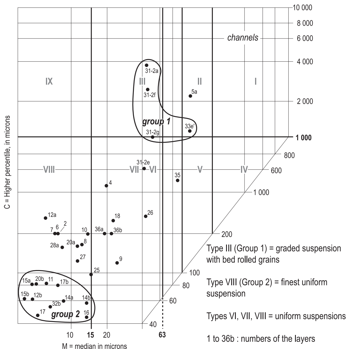
Fig. 3: Oued Noun at Fort Oued Noun: Passega CM diagram of Unit 2 (after R. Passega & R. Byramjee, 1969; P. Guery, 2000; J. Mathieu, to be published).
