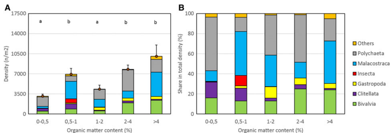
Fig. 9. Absolute (A) and relative (B) numbers of individuals per major taxonomic group with organic matter content (% DW). Average total densities \pm standard error for clusters of times 2 increasing organic matter contents; significant differences in total densities are indicated with different characters.
