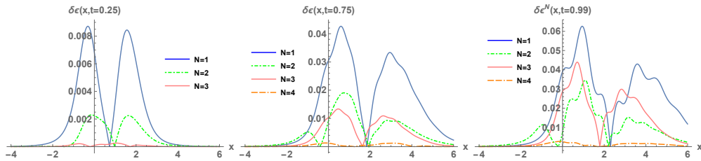
Figure 6: Differences in consecutive estimates \delta\epsilon^N(x, t) (see (6)) at t = 0.25 (left), t = 0.75 (center) and t = 0.99 (right), and for orders of truncation as indicated. The plots correspond to Example 5.2.
