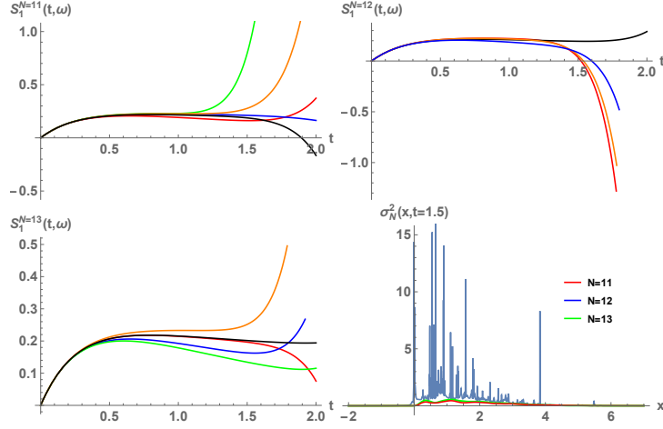
Figure 10: Random trajectories of S_1^N(t, \omega) for N = 11, 12 and 13 . For N = 12 , observe that some trajectories vanish very close to t = 1.5 , while for N \neq 12 the trajectories remain away from 0. The plot in the bottom right panel shows the corresponding empirical estimates of \sigma_N^2(x, t = 1.5) . Observe that for N = 11 and N = 13 the variances are small, while \sigma_{N=12}^2 is large (the range has been restricted to 15). This figure corresponds to Example 5.3.
