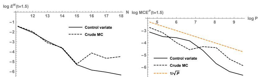
Figure 14: Left: error E^N(t = 1.5) (see (8)). Right: sampling error MCE^P(t = 1.5) (see (10)) with the number of realizations P . This figure corresponds to Example 6.1.
