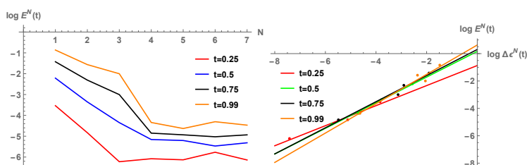
Figure 7: Left: error E^N(t) in (8), for different times as indicated. Right: relation between \log E^N(t) and \log \Delta\epsilon^N(t) , for t = 0.25, 0.5, 0.75 and 0.99 . Also reported are linear regressions. This figure corresponds to Example 5.2.
