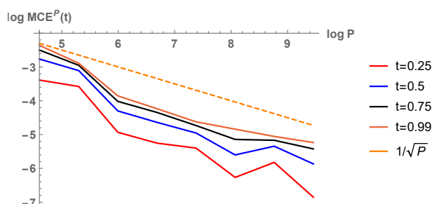
Figure 8: Sampling error (10) with the number of realizations P , for different times as indicated. This figure corresponds to Example 5.2.
