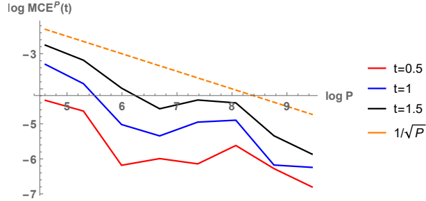
Figure 4: Sampling error (10) with the number of realizations P , for different times as indicated. This figure corresponds to Example 5.1.
