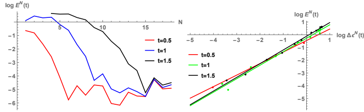
Figure 3: Left: error E^N(t) (see (8)), for different times as indicated. Right: relation between \log E^N(t) and \log \Delta\epsilon^N(t) , for t = 0.5 , t = 1 and t = 1.5 . Also reported are linear regressions. This figure corresponds to Example 5.1.
