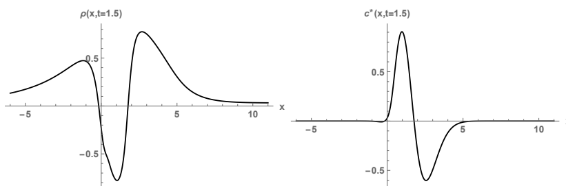
Figure 15: Left: correlation coefficient. Right: control coefficient. This figure corresponds to Example 6.1.
