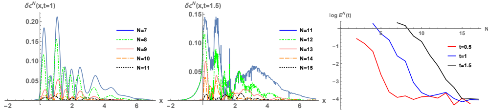
Figure 11: Differences in consecutive estimates \delta \epsilon^N(x, t) at t = 1 (left) and t = 1.5 (center), with orders of truncation as indicated. The last plot presents the errors E^N(t) (see (8)), for different times as indicated. This figure corresponds to Example 5.3.
