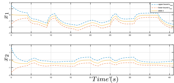
(a) State and estimated bounds
