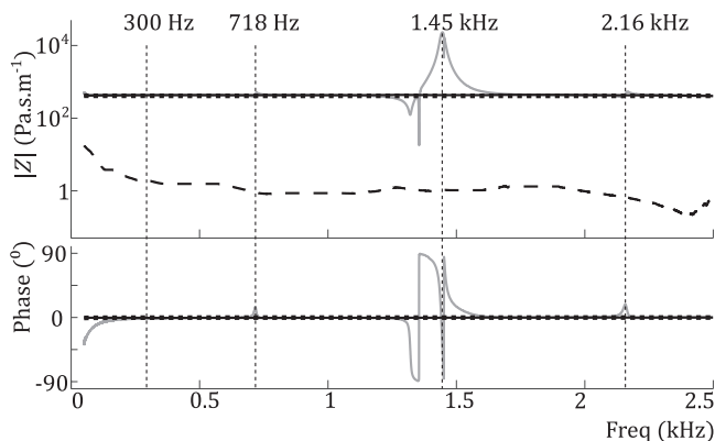
FIG. 3. Averaged value of the characteristic impedance Z_c in the plastic pipe (solid gray), calculated using the impedance measurements Z_{1,\text{plastic}} and Z_{2,\text{plastic}} , and smoothed using a median filter (solid black). The dotted black lines show the theoretical value Z_c^{\text{th}} , for temperature and relative humidity equal to average experimental values: 21.9 °C and 59%. In the upper figure, the dashed black curve shows the standard deviation of the 100 estimates of Z_c .
