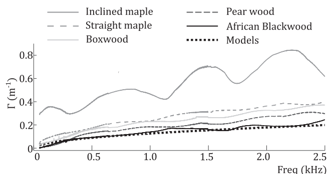
FIG. 6. Attenuation factors in the pipes made of maple, boxwood, pear wood, and African Blackwood before polishing (solid and dashed curves). The five superimposed dotted black curves show theoretical curves for smooth and non-porous pipes with same dimensions as the pipes of the corpus and with visco-thermal losses inside the bore. They are calculated using experimental values of temperature and relative humidity.
