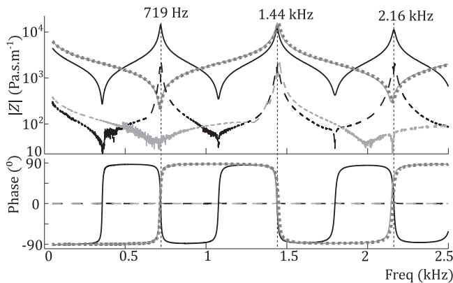
FIG. 2. Averaged input impedances (pressure divided by longitudinal velocity) of the closed plastic pipe, while the length of the air column is L_1 = 238.5 mm (solid black) and L_2 = L_1/2 (solid gray). The dotted gray line shows the averaged input impedance Z_{2,\text{plastic}} , after correction, so that the average distance between the zeroes of its phase and those of Z_{1,\text{plastic}} is minimized. The dashed lines show the standard deviations of the ten measurements of Z_{1,\text{plastic}} (black) and Z_{2,\text{plastic}} (gray).
