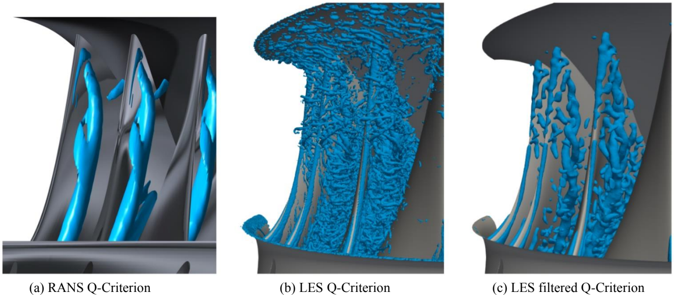
Fig. 6 Comparison between RANS and LES results at OP4.
