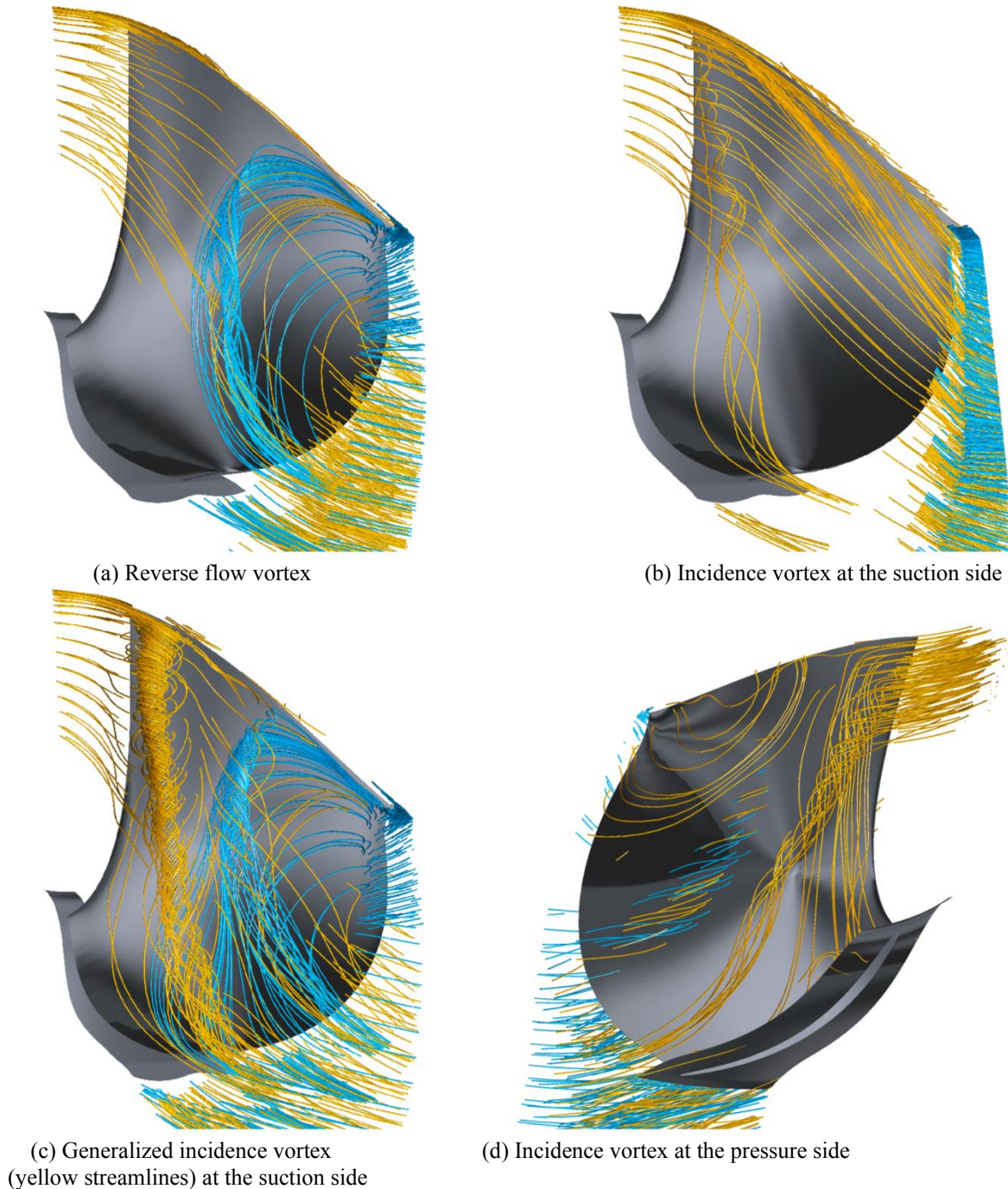
Fig. 3 Four types of vortices with the velocity streamlines: the yellow ones come from the inlet and the blue ones from the outlet.
