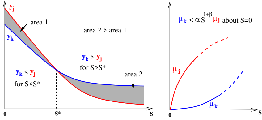
Fig. 1. Graphical illustration of sufficient conditions for overyielding.
