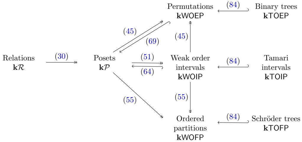
FIGURE 3. A roadmap through the different Hopf algebras studied in this paper. An arrow \rightarrow indicates a quotient Hopf algebra, while an arrow \hookrightarrow indicates a Hopf subalgebra. The label on each arrow refers to the corresponding proposition.
