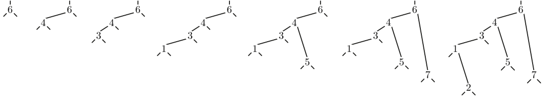
FIGURE 9. Binary search tree insertion of the permutation \sigma = 2751346 .
