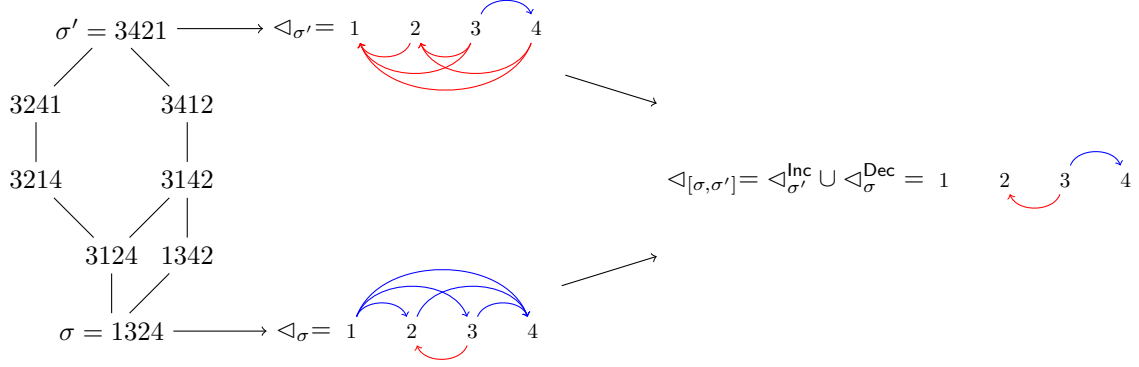
FIGURE 5. A Weak Order Interval Poset (WOIP).
