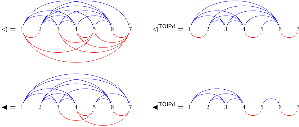
FIGURE 14. The TOIP deletion.
