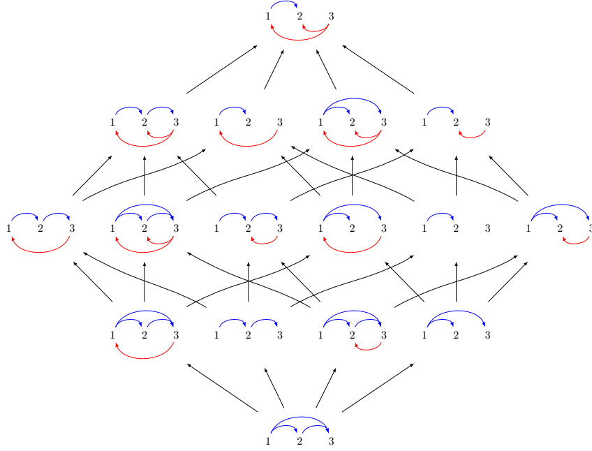
FIGURE 1. Interval corresponding to a product of relations.
