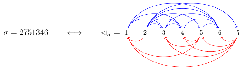
FIGURE 4. A Weak Order Element Poset (WOEP).
