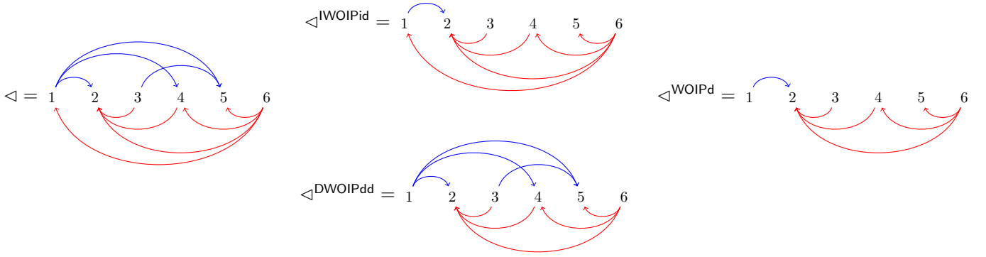
FIGURE 8. The IWOIP increasing deletion and the DWOIP decreasing deletion.
