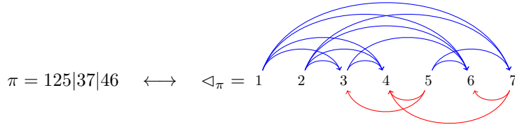
FIGURE 7. A Weak Order Face Poset (WOFP).
