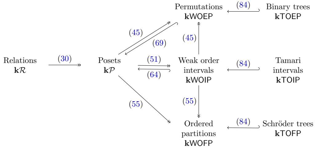
FIGURE 3. A roadmap through the different Hopf algebras studied in this paper. An arrow \rightarrow indicates a quotient Hopf algebra, while an arrow \leftrightarrow indicates a Hopf subalgebra. The label on each arrow refers to the corresponding proposition.
