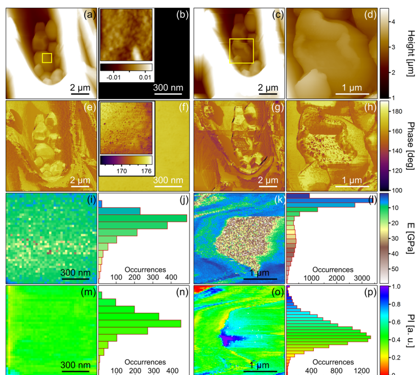
Figure 5. Mechanical properties of starch granules through nanomechanical force measurements on a single granule. A comparison between the unablated outer surface (a,b,e,f,i,j,m,n) and the region of the inner surface after ablation (c,d,g,h,k,l,o,p) reveals differences in topography, E and, PI. In (a,c), the yellow squares on the topographical images mark the zoomed regions in the outer surface (b,f,i,j,m,n) and inner surface (d,h,k,l,o,p), respectively. The phase images (e–h) provide additional detail to the topographical images (a–d), where greater roughness is observed in the inner surface (h). The E mapping and the resulting distribution histogram of the inner surface, (k,l), respectively, is a factor of 3 larger than the outer surface, (i,j), respectively. The PI mapping and resulting distribution histogram of the inner surface (o,p), respectively, is a factor of 2 larger than the outer surface (m,n), respectively.
