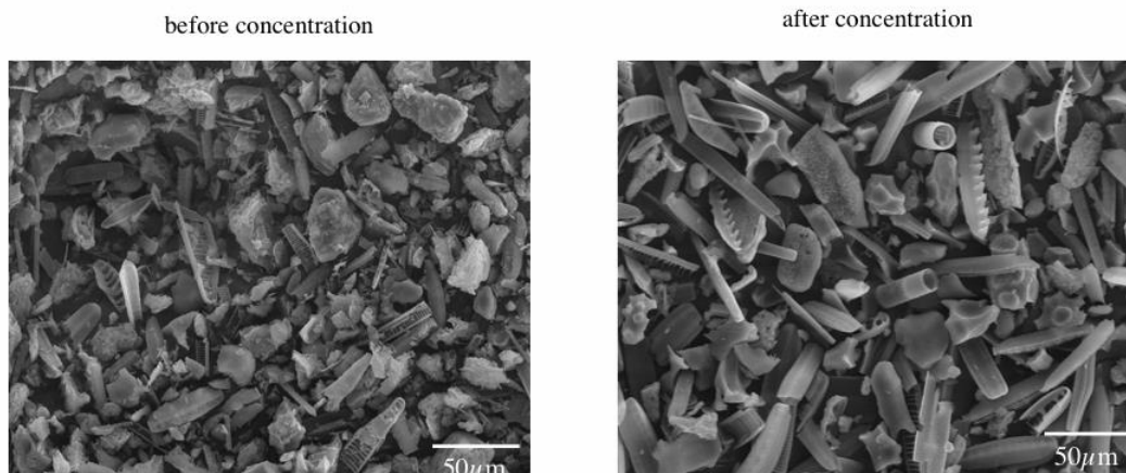
Figure 2 SEM photo performed on Lubbock Lake LL65-2A sample before and after concentration with the same magnification ( \times 400 ). Note the disappearance of clay after concentration treatment.
