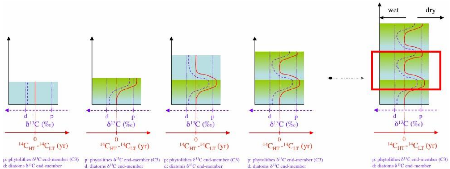
Figure 5 Schematic view of the succession phases of Mustang Spring accumulation, with representations of \delta^{13}\text{C} and ^{14}\text{C}_{\text{HT}}-^{14}\text{C}_{\text{LT}} . Since the \delta^{13}\text{C} scale is not numerically defined, the \delta^{13}\text{C} representation is for both bulk and concentrate and both HT and LT fractions. Likewise, ^{14}\text{C}_{\text{HT}}-^{14}\text{C}_{\text{LT}} is for both bulk and concentrate. From left to right: 1 - a wet episode with diatomite accumulation (blue) characterized by ^{14}\text{C}_{\text{HT}}-^{14}\text{C}_{\text{LT}} close to zero and a relatively heavy \delta^{13}\text{C} close to the diatom end-member; 2 - a dry episode with soil development (green) into diatomite layers characterized by increasing ^{14}\text{C}_{\text{HT}}-^{14}\text{C}_{\text{LT}} and decreasing \delta^{13}\text{C} towards the phytolith end-member; 3 - a new wet episode with diatomite accumulation on the previous soil characterized by a return of ^{14}\text{C}_{\text{HT}}-^{14}\text{C}_{\text{LT}} to 0 and an increase of \delta^{13}\text{C} , then another dry period, and so on to show the Mustang Spring series. The red rectangle in the last panel shows the Mustang Spring fraction that we study here.
