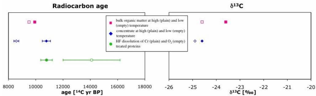
Figure 3 Lubbock Lake. Left: ^{14}\text{C} results according to the applied protocol: pink squares are for bulk organic matter at low (empty square) and high (plain square) temperatures, blue diamonds are for concentrate at low (empty diamond) and high (plain diamond) temperatures, green circles are for HF dissolution of Cr (plain circle) and \text{O}_2 (empty circle) extracts. See text and Figure 1 for details on protocol. Right: \delta^{13}\text{C} results according to the applied protocol. Same symbols as left panel.
