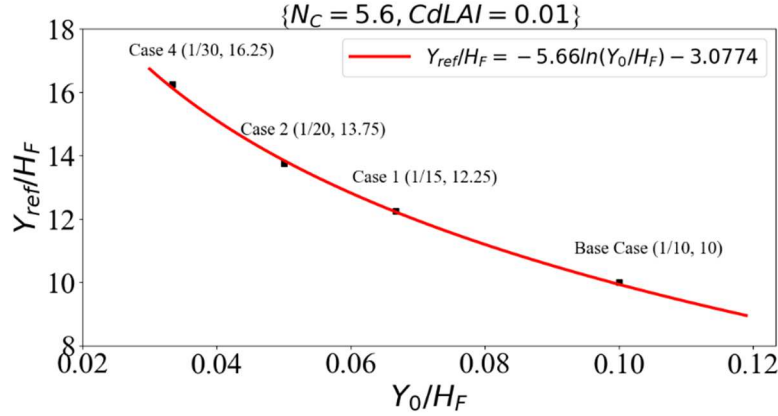
Fig. 7. Mathematical expression and best-fit curve for scaling Y_{ref} .
