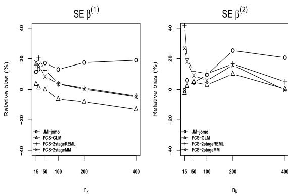
FIG. 6. Robustness to the cluster size: estimate of the relative bias for the SE estimate for \widehat{\beta}^{(1)} (left), \widehat{\beta}^{(2)} (right) according to n_k for each MI method. The estimated relative bias is calculated by the difference between the model SE and the empirical SE, divided by the empirical SE. Criteria are based on 500 incomplete datasets.
