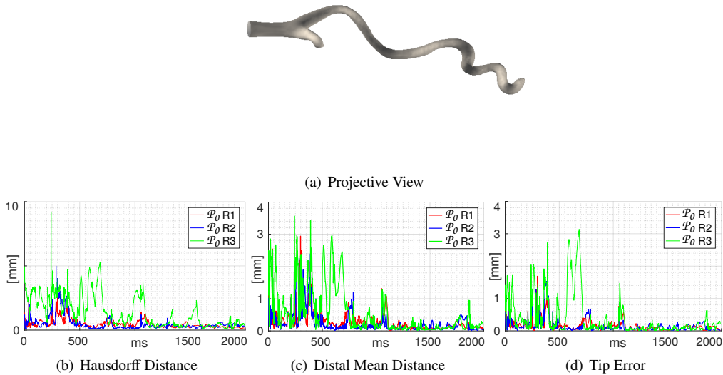
Figure 16: Evaluation Metrics for Synthetic Vessel Geometry. Metrics provided for filter parameters combination \mathcal{P}_0 . Whenever R is small (green graph), reconstruction appears less accurate due to the confidence given to observations which have an intrinsic uncertainty in depth direction.
