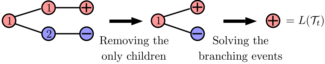
FIGURE 4. Solving the determination tree.
