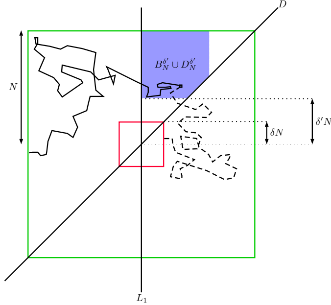
FIGURE 2. A random walk started in B_N^{\delta'} (blue area) has a probability of order \log(\delta')/\log(\delta) of hitting \Lambda_{\delta N} (red boundary) before \Lambda_N^c (green boundary) (dashed trajectory). In particular, as \delta \rightarrow 0 , it will most likely hit the green boundary before the red one (solid trajectory).
