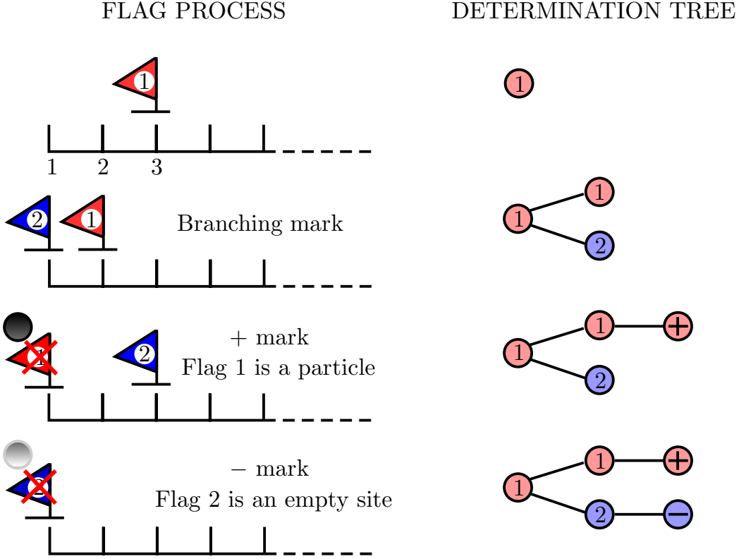
FIGURE 3. An example of construction of the determination tree. Each time a boundary mark is encountered by one of the flags in the process \mathcal{A} , the tree is updated accordingly, by adding two children (for a branching mark) to each node with the affected flag's label, or one single child labelled \pm (for a \pm mark).
