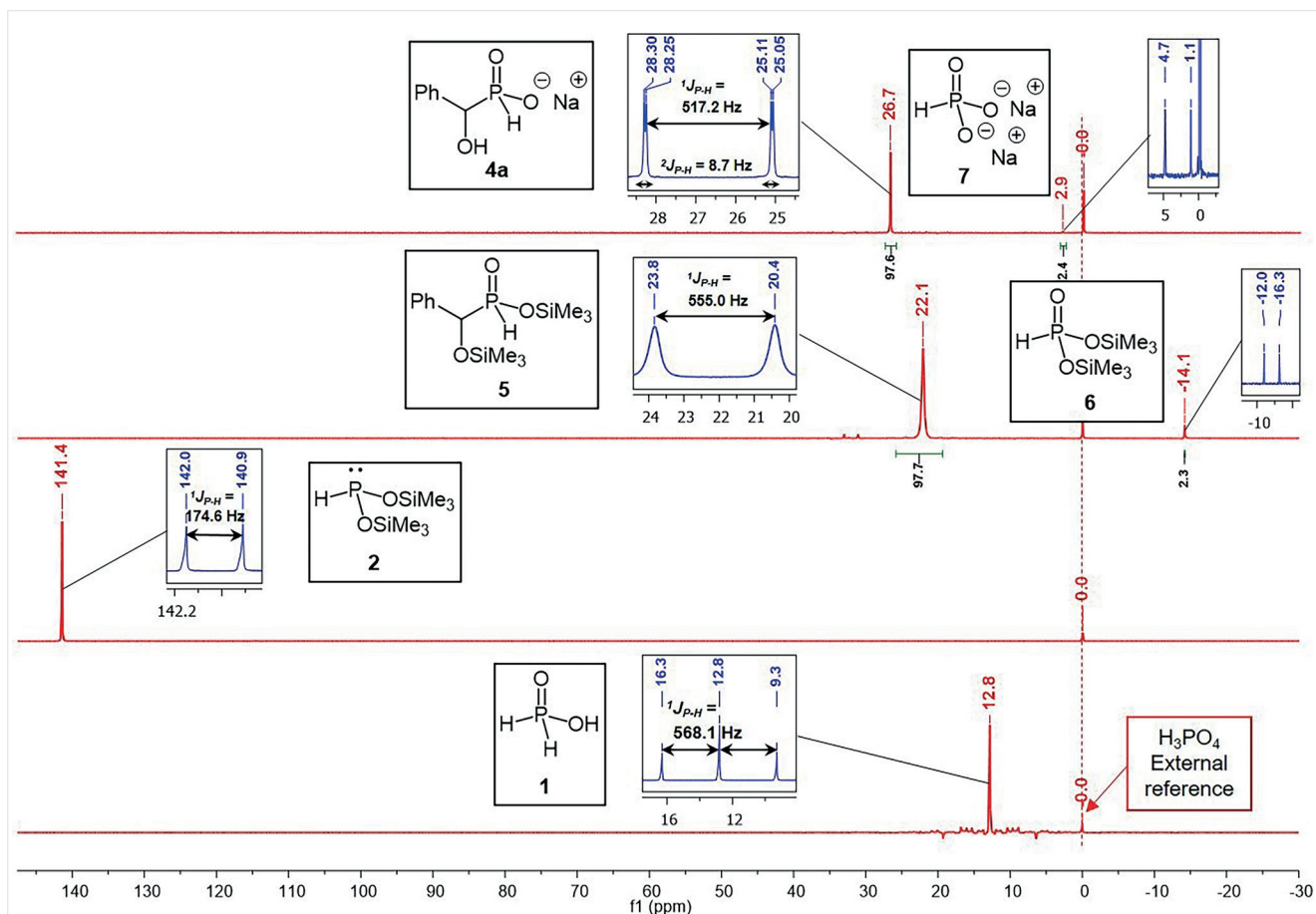
Figure 1 ^{31}\text{P}[^1\text{H}] (in red) and ^{31}\text{P} (in blue) NMR monitoring of the Abramov reaction between hypophosphorous acid ( 1 ; 1 equiv) and benzaldehyde ( 3a ; 1 equiv) in the presence of BSA (2 equiv)
