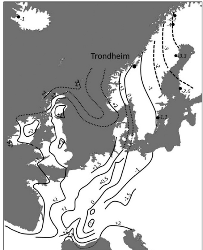
Fig. 5. Deviation of the \delta^{18}O_w from -9\% (the yearly weighted precipitation in Trondheim in 2013 = -8.8\% ; the mean temperature in 2004–2014 converted to \delta^{18}O_w = -9.3\% ) based on a compilation by C. Chenery. British Geological Survey (based on Darling et al. (2003) and Lecolle (1985)).
