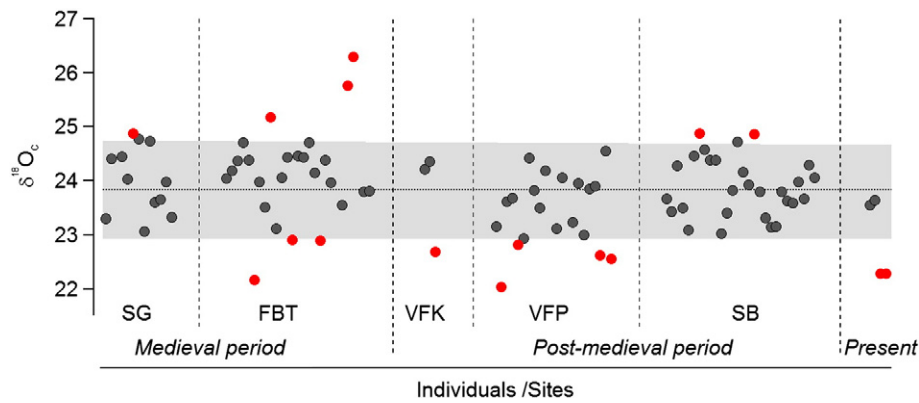
Fig. 4. Oxygen isotopic composition of the M3 teeth of the individuals excavated at Trondheim (column 6, Table 2). The shaded area corresponds to an intra-population variability of 0.9‰. The red dots correspond to the individuals who may have migrated to Trondheim after the age of 14 years old. SG: Søndregate; FBT: Folkebibliotekstomten; VFK: Vår frue kirke; VFP: Vestfrontplassen; SB: Servicebygget.
