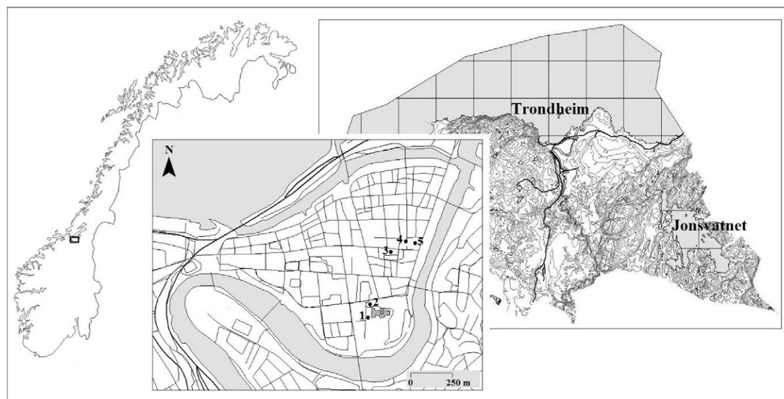
Fig. 1. Maps showing Norway with the location of Trondheim (left), the municipality of Trondheim with Lake Jonsvatnet (right), and the town centre of Trondheim with the five archaeological sites providing the skeletal material for this study (front): 1. Vestfrontplassen (1585–1897); 2. Servicebygget (1585–1897); 3. Vår Frue Kirke (16th–mid-19th century); 4. Søndregate (mid-12th century–1531); 5. Folkebibliotekstomten (1175–1275).
