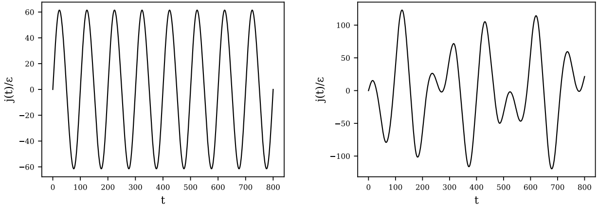
Figure 3: Instantaneous conductivity \frac{j_{\alpha,\beta}^\varepsilon(t)}{\varepsilon} in the Bloch oscillations regime ( \varepsilon = 10^{-2} , \frac{1}{\varepsilon} \ll t ). We take e_\alpha = b_1 . The left figure is with e_\beta = b_1 + b_2 , the right one with e_\beta = b_1 + \frac{1+\sqrt{5}}{2}b_2 .
