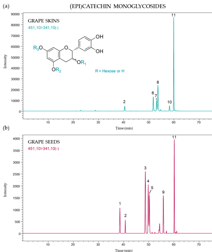
Figure 2. (Epi)catechin monoglycoside profile of (a) skins and (b) seeds from Vitis vinifera grapes using multiple reaction monitoring (MRM) [451 \rightarrow 341].
