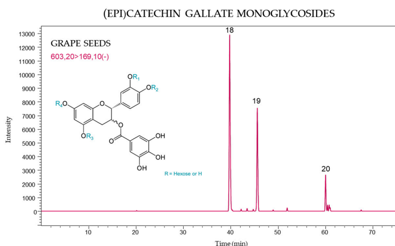
Figure 4. (Epi)catechin gallate monoglycoside profile of V. vinifera grape seeds using MRM [603 → 169].
