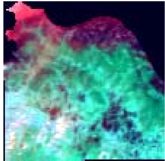
Figure 4. Karawang-West Java Using MODIS Satellite, in size (100x100) pixels
