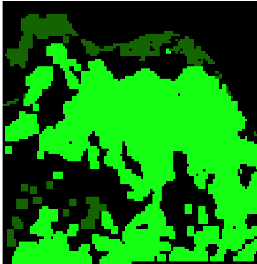
Figure 6. Mapping of Karawang Rice Field, in size (100x100) pixels
