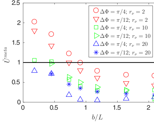
FIG. 7. Normalized average velocity \tilde{U}^{meta} as a function of the cilia spacing b/L in the y-direction for three values of the viscosity ratio r_v , for antiplectic metachronal waves with \Delta\Phi = \pi/4 and \Delta\Phi = \pi/12 . The solid black line represents the value of \tilde{U}^{lub} . The value of the PCL depth is set to h/L = 0.91 .
