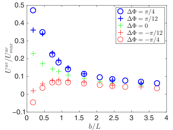
FIG. 4. Normalized average velocity U^* = U^{\text{av}}/U_{\text{max}}^{\text{av}} as a function of the cilia spacing b/L in the y -direction for different phase lags \Delta\Phi . The value of r_v is set to 10, and the PCL depth to h/L = 0.91 .
