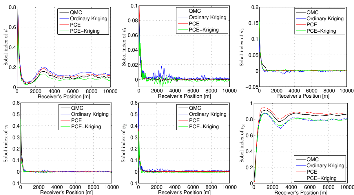
Figure 8: Variation of the Sobol sensitivity indices of all random variables in terms of the source-station distance for f = 10 Hz. Black, blue, red and green curves represent the results obtained by QMC, Kriging, PCE and PCE-Kriging methods, respectively.
