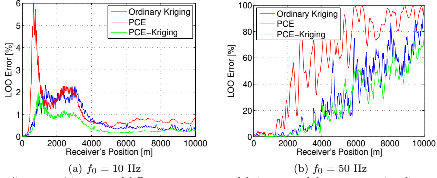
Figure 6: LOO errors (in percent) in terms of different surrogate models in terms of the source-station distance for f_0 = 10 Hz(a) and f_0 = 50 Hz(b).
