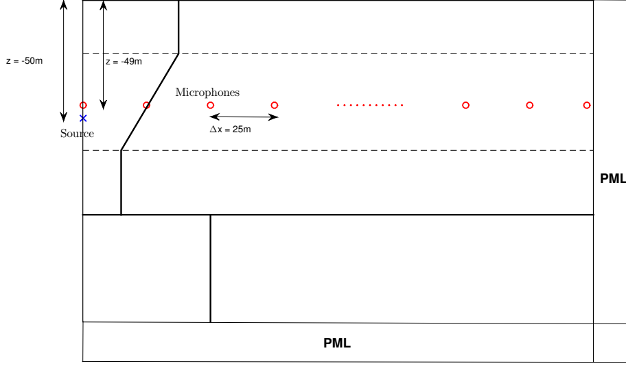
Figure 2: The configuration of the source and the microphones.
