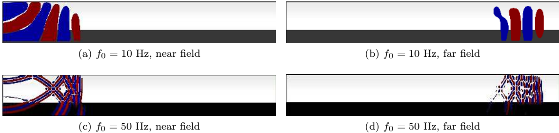
Figure 5: Snapshots of the wave field near (a,c) and far (b,d) from the source for f_0 = 10 Hz (a,b) and f_0 = 50 Hz (c,d).
