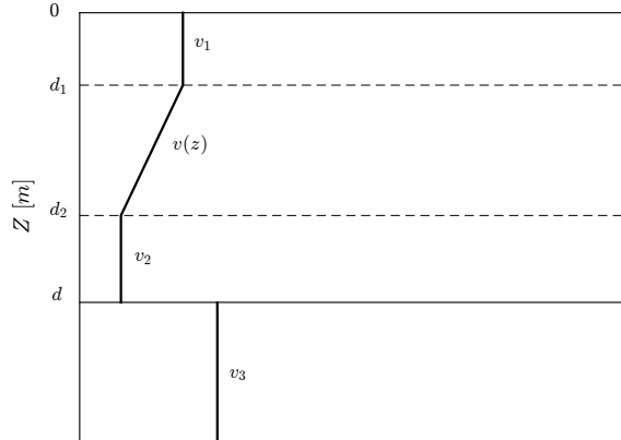
Figure 1: Shallow water environment with a four-layer sound speed profile v(z) .
