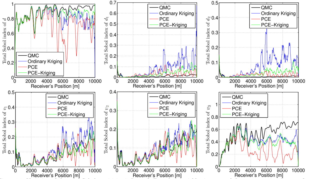
Figure 11: Variation of the total Sobol sensitivity indices of all random variables in terms of the source-station distance for f = 50 Hz. Black, blue, red and green curves represent the results obtained by QMC, Kriging, PCE and PCE-Kriging methods, respectively.
