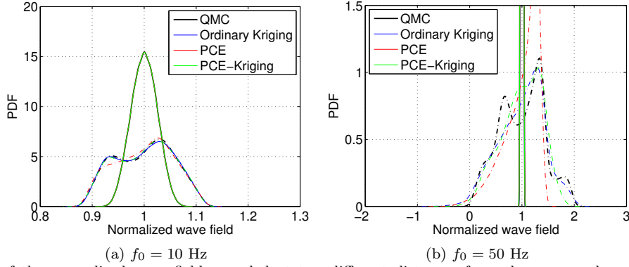
Figure 7: PDFs of the normalized wave field recorded at two different distances from the source whose central frequency is 10 Hz(a) and 50 Hz(b). Black, blue, red and green curves represent the results obtained by QMC, Kriging, PCE and PCE-Kriging methods, respectively. Solid and dashed dotted lines correspond to |\mathbf{r} - \mathbf{r}^0| = 1 m and |\mathbf{r} - \mathbf{r}^0| = 5000 m.
