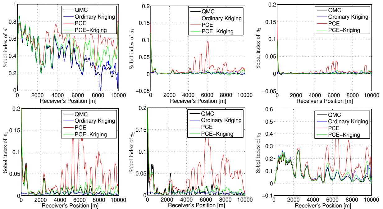
Figure 10: Variation of the Sobol sensitivity indices of all random variables in terms of the source-station distance for f = 50 Hz. Black, blue, red and green curves represent the results obtained by QMC, Kriging, PCE and PCE-Kriging methods, respectively.
