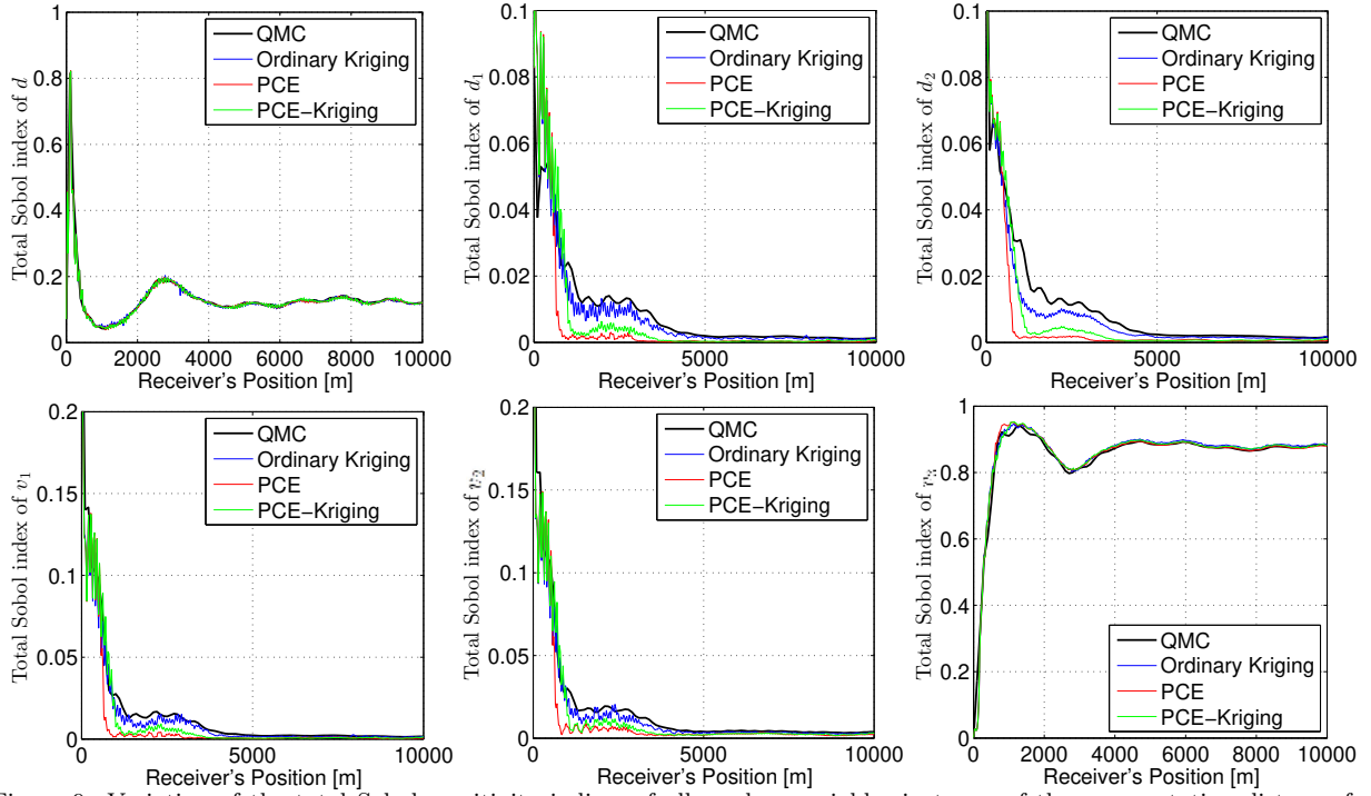
Figure 9: Variation of the total Sobol sensitivity indices of all random variables in terms of the source-station distance for f = 10 Hz. Black, blue, red and green curves represent the results obtained by QMC, Kriging, PCE and PCE-Kriging methods, respectively.
