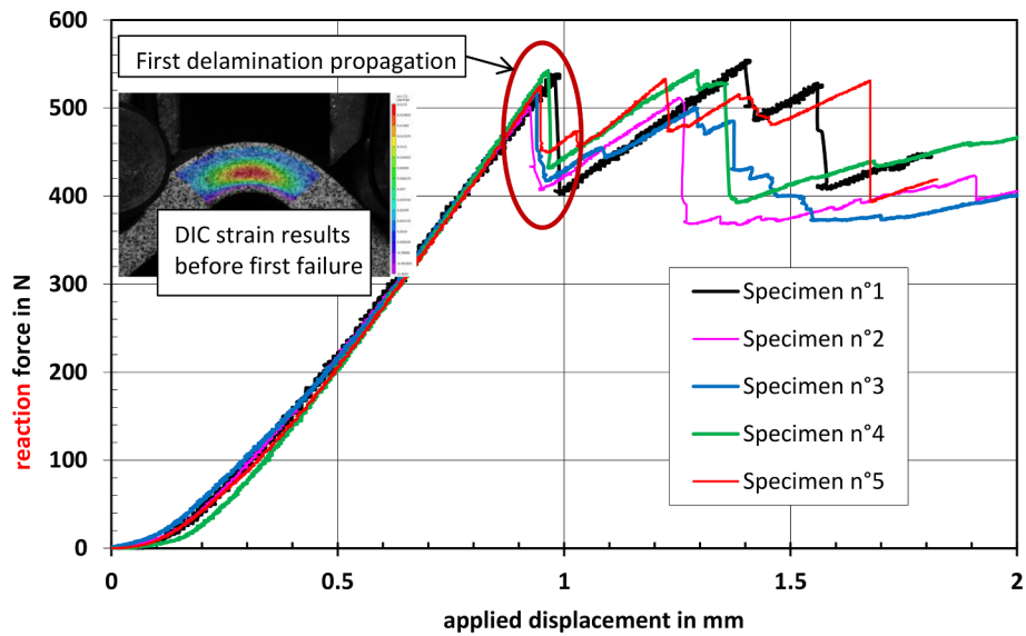
Fig. 9. 4PLB experimental test results: force versus displacement behavior (see the web version in which each curve has a specified color).
