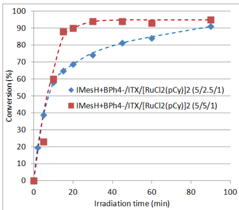
Figure 4: Nb conversion as a function of the irradiation time for the miniemulsion ROMP with the catalytic system \text{IMes}^+\text{BPh}_4^-/\text{ITX}/[\text{RuCl}_2(\text{pCy})]_2 (5/2.5/1 equiv.) blue curve and (5/5/1 equiv.) red curve; irradiance 25 mW/cm 2 ; sonication time 10 min.
