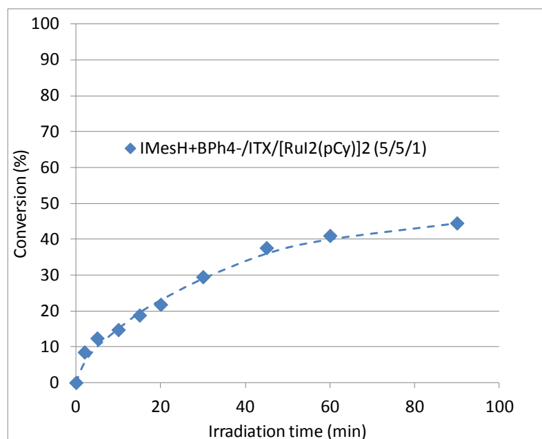
Figure 5: Nb conversion as a function of the irradiation time for the miniemulsion ROMP with the catalytic system \text{IMesH}^+\text{BPh}_4^-/\text{ITX}/[\text{RuI}_2(\text{pCy})]_2 (5/5/1 equiv.); irradiance 25 \text{mW}/\text{cm}^2 ; sonication time 10 min.
