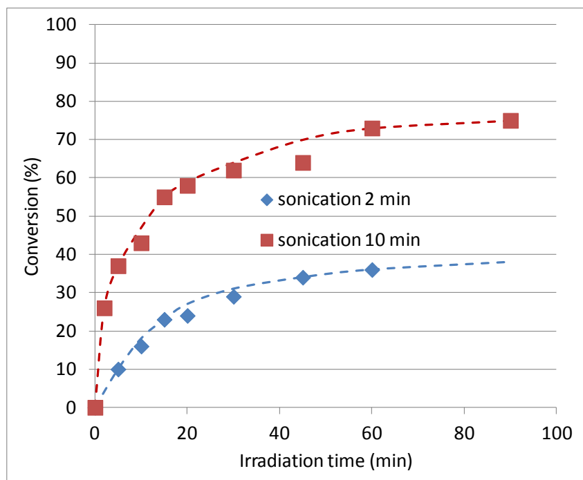
Figure 2: Nb conversion as a function of the irradiation time for the miniemulsion ROMP with the catalytic system \text{IMes}^+\text{BPh}_4^-/\text{ITX}/[\text{RuCl}_2(\text{pCy})_2] (5/2.5/1 equiv.); irradiance 130 \text{ mW/cm}^2 ; in blue after 2 min of sonication and after 10 min of sonication in red.
