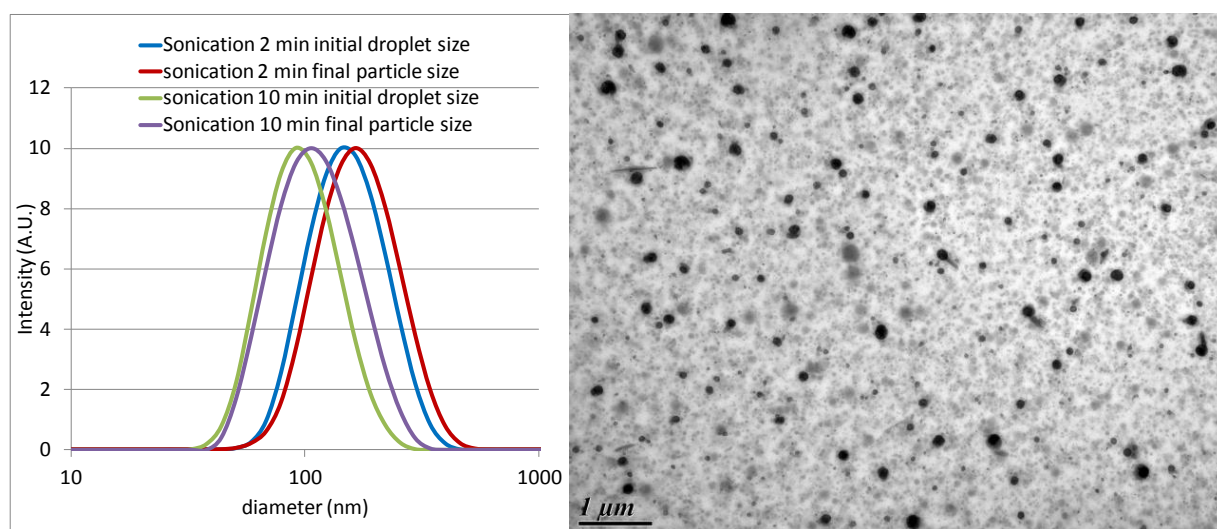
Figure 3: Left: initial droplet size and final particle size measured by DLS for the miniemulsion ROMP with the catalytic system \text{IMes}^+\text{BPh}_4^-/\text{ITX}/[\text{RuCl}_2(\text{pCy})_2] (5/2.5/1 equiv.); irradiance 130 \text{ mW/cm}^2 for 2 min and 10 min of sonication. Right: TEM picture of the final particles for a sonication time of 10 min.
