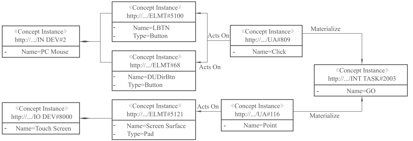
Fig. 23 Instances of our ontology concepts used to rewrite labels
