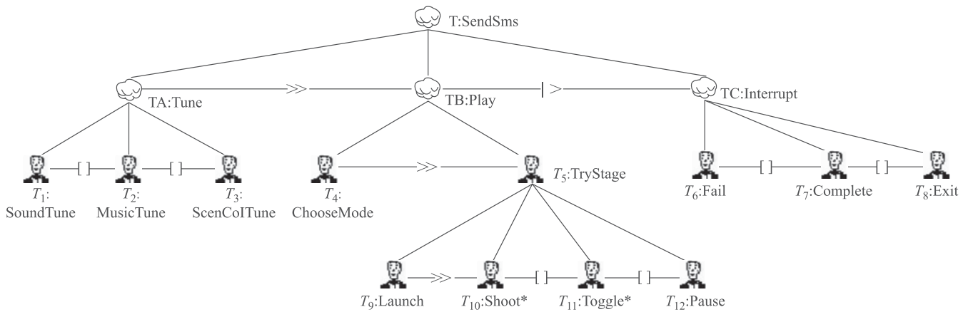
Fig. 17 “Marble Legend” game abstract task model
