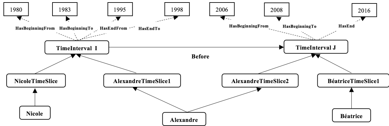
Figure 3: An instantiation of the extended 4D-fluents model in OWL 2.
