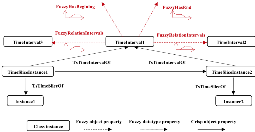
Figure 5: The extended 4D-fluents model in Fuzzy-OWL 2.
