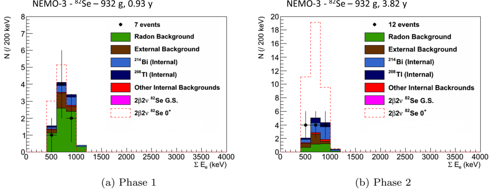
Figure 12: Total electron energy distributions after selection for the 2\nu\beta\beta(0_{g_s}^+ \rightarrow 0_1^+) transition, for Phase 1 in Figure 12(a) and Phase 2 in Figure 12(b). Experimental data events are compared to the MC simulation for the different backgrounds. The dotted red line represents the simulated signal for a half-life of 3 \times 10^{20} years.
