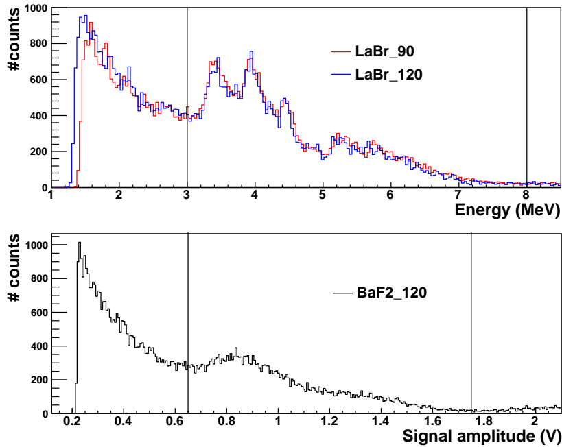
Figure 3. Energy spectra obtained with the two \text{LaBr}_3 detectors, LaBr_90 and LaBr_120 (top), and the BaF2_120 detector (bottom). The 3–8 MeV energy selection window is shown in both graphs.
