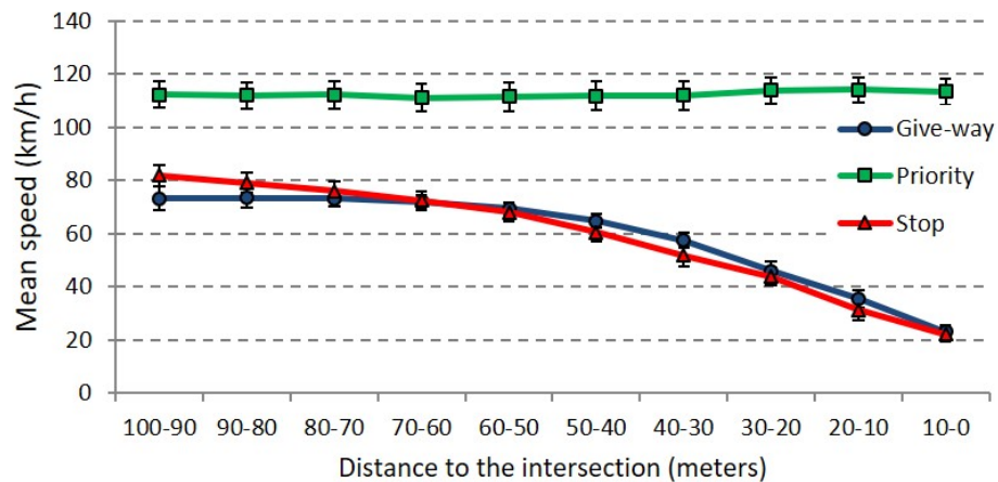
Figure 4: Average speed during the intersection approach for each of the three priority rules (Give way, Stop and Priority).
