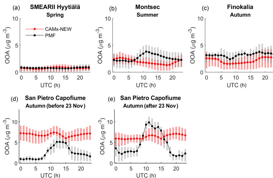
Figure 7. Diurnal variations of modeled OOA components by CAMx-NEW and PMF studies in rural or remote sites. The lines represent the average value of modeled and measured OOA. Bars represent 25th and 75th percentiles of hourly data.
