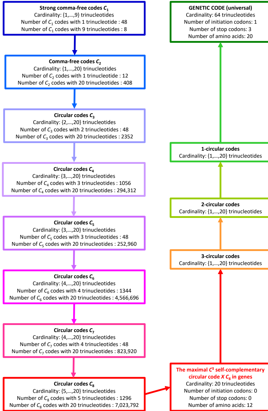
FIGURE 4. A combinatorial hierarchy of circular (4-circular) trinucleotide codes C_p , where p is the maximal path length associated with the graph \mathcal{G}(C_p) , and k -circular trinucleotide codes, where k \in \{1, 2, 3\} (see Theorem 4.1 with n = 4 and \ell = 3 , and Corollary 4.2).
