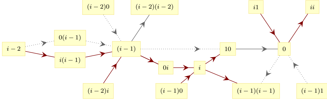
FIGURE 11. The changes in the middle component in the proof of (H)(1). All grey arcs belong to \mathcal{G}(Y_i) , and all plain arcs belong to \mathcal{G}(Y_{i+1}) .
