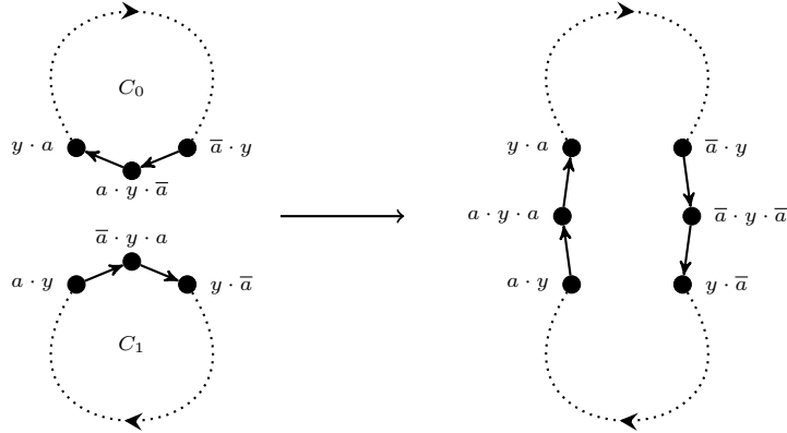
FIGURE 7. Schematic view of the merging of two cycles in the proof of (E1).
