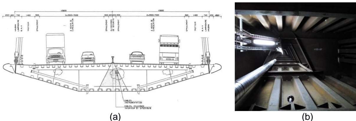
Figure 2 - Bridge of Normandy: (a) cross section, (b) inside of the box.
