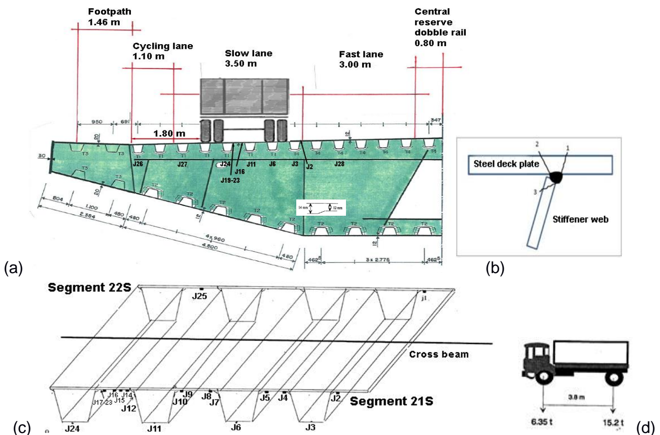
Figure 3 – (a) Bridge of Normandy, transverse cross section, (b) detail sensitive to fatigue, (c) stain gauges, and (d) test truck.
