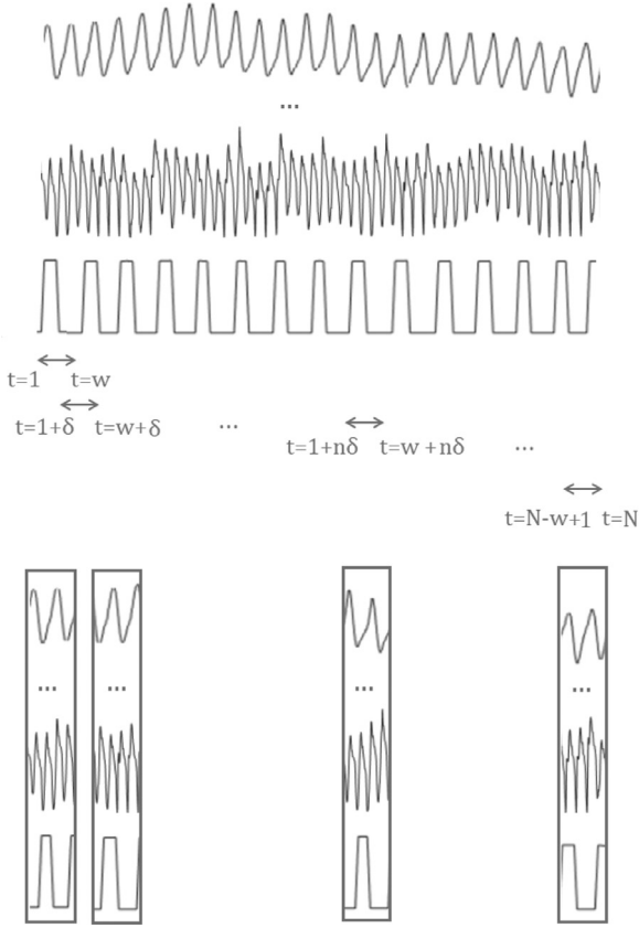
Fig. 2. Segmentation of telemetry into overlapping windows.
