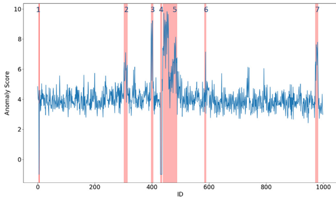
Fig. 5. Anomaly scores obtained with ADDICT for the dataset with ground-truth marked by red background and the shift-invariance option enabled with \tau_{\max} = 5 . (For interpretation of the references to colour in this figure legend, the reader is referred to the web version of this article.)
