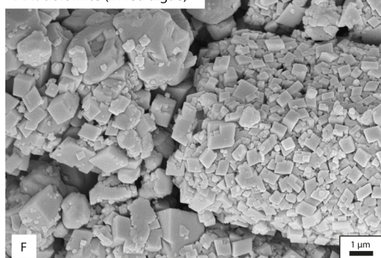
M4: dolomite (in red algae)
