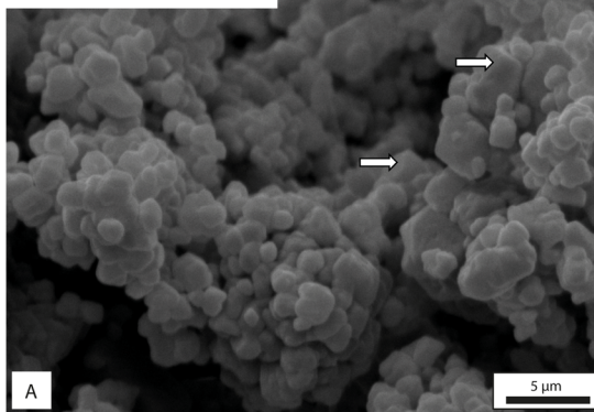
M2: densely packed micrite
