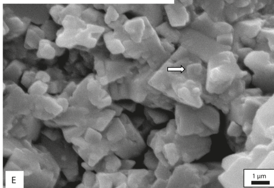
M3: subhedral to euhedral micrite
