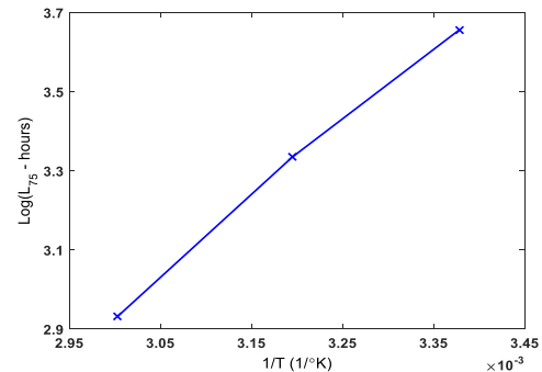
Fig. 9. Linear variation of \text{Log}(L) versus 1/T ( T in K) at J = 11.25 mA / cm 2
